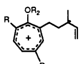
14a R_2 = H or - , R_1 = CH_3 , R_2 = H 14b R_2 = H or - , R_1 = H , R_2 = CH_3
