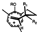
13a R_2 = H or - , R_1 = CH_3 , R_2 = H 13b R_2 = H or - , R_1 = H , R_2 = CH_3
