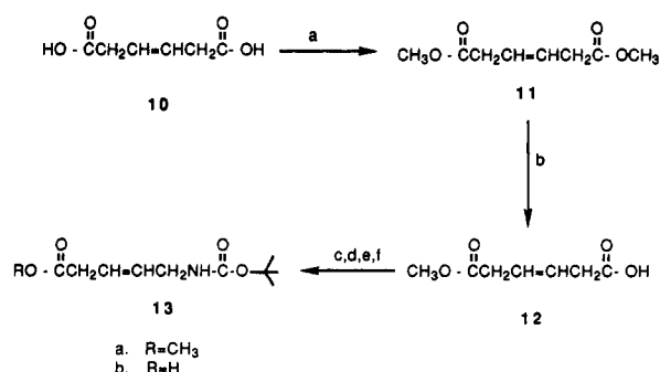
Scheme III. a Synthesis of N -Boc-5-Amino-3-pentenoic Acid Unit Serving as the Spacer for IIIa-c
