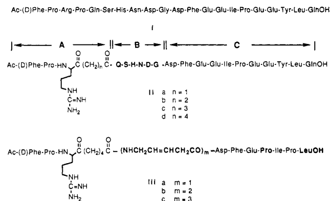
Figure 1. Structure of [Ac-(D)Phe 45 ,Arg 47 ]hirudin45-65 (I), hirutinin 1-4 (IIa-d), and modified hirutinin 4 (IIIa-c).
