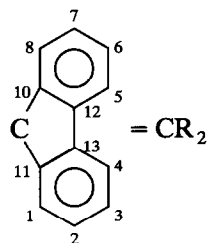
Scheme 1.
