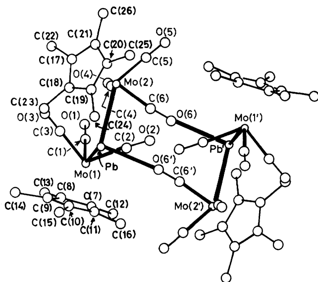
Figure 2. The molecular structure of [\{\text{Pb}\{\text{Mo}(\eta\text{-C}_5\text{Me}_5)(\text{CO})_3\}[\text{Mo}(\eta\text{-C}_5\text{Me}_5)(\text{CO})_2(\mu\text{-CO})\}]_2] (3), showing the atom numbering scheme (primed atoms correspond to \bar{x}, 1 - \bar{y}, \bar{z} )
