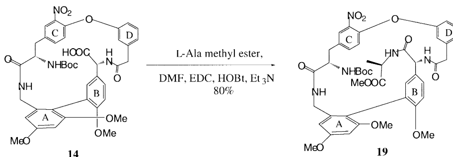
Scheme 5.
