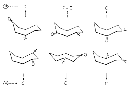
Scheme I. Alcohol Configurations a from "P"-Controlled Reduction of Different 3- tert -Butylcyclooctanone Conformers
