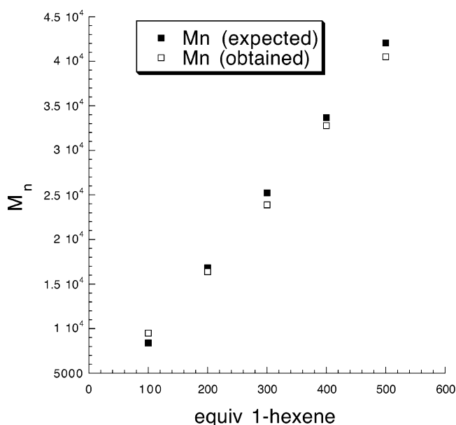
Figure 3. Molecular weights of poly[1-hexene] obtained with 3 mM \{[ArClN_2NMe]ZrMe\}\{B(C_6F_5)_4\} as the initiator in chlorobenzene at 0 °C.
