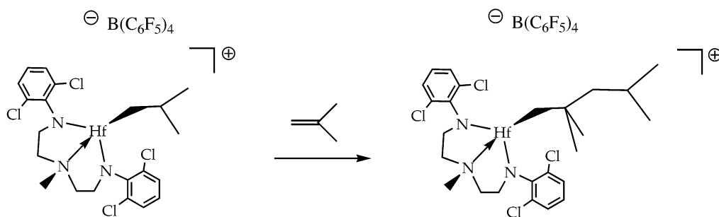
Scheme 2. Insertion of Isobutene into \{[ArClN_2NMe]Hf(i-Bu)\}^+\{B(C_6F_5)_4\}^-
