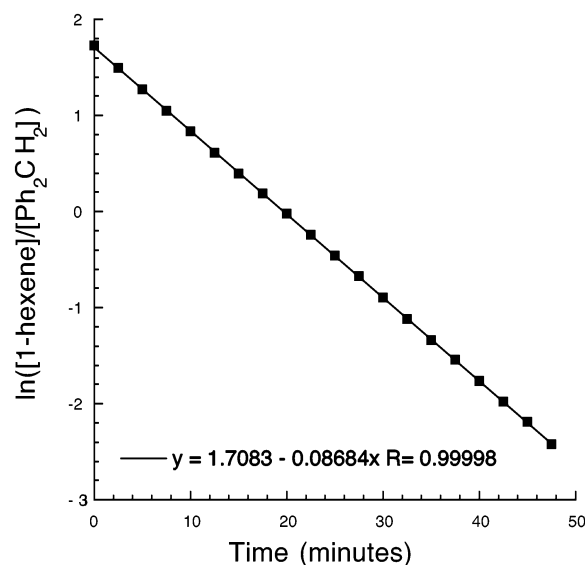
Figure 2. Consumption of the final 13% of 100 equiv of 1-hexene at 0 °C by 0.006 M \{[ArClN_2NMe]HfMe\}\{B(C_6F_5)_4\} (formed by the activation of [ArClN_2NMe]HfMe_2 with \{Ph_3C\}\{B(C_6F_5)_4\} ).
