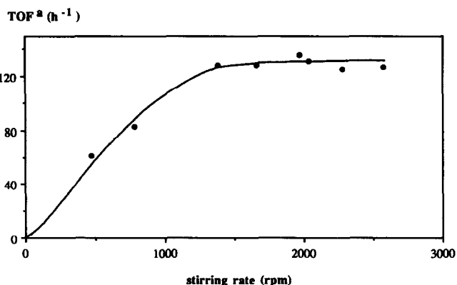
Fig. 3. Influence of the stirring rate on the turn-over frequency TOF of hydroformylation of oct-1-ene. ( 1 , 0.16 mmol; oct-1-ene, 64 mmol; TPPTS, 2.88 mmol; H_2O , 110 ml; ethanol, 40 ml; P = 0.5 MPa ( [H_2]/[CO] = 1 ); T = 80^\circ C , t = 15 h). The turnover frequency was measured between 0.5 and 1 h.
