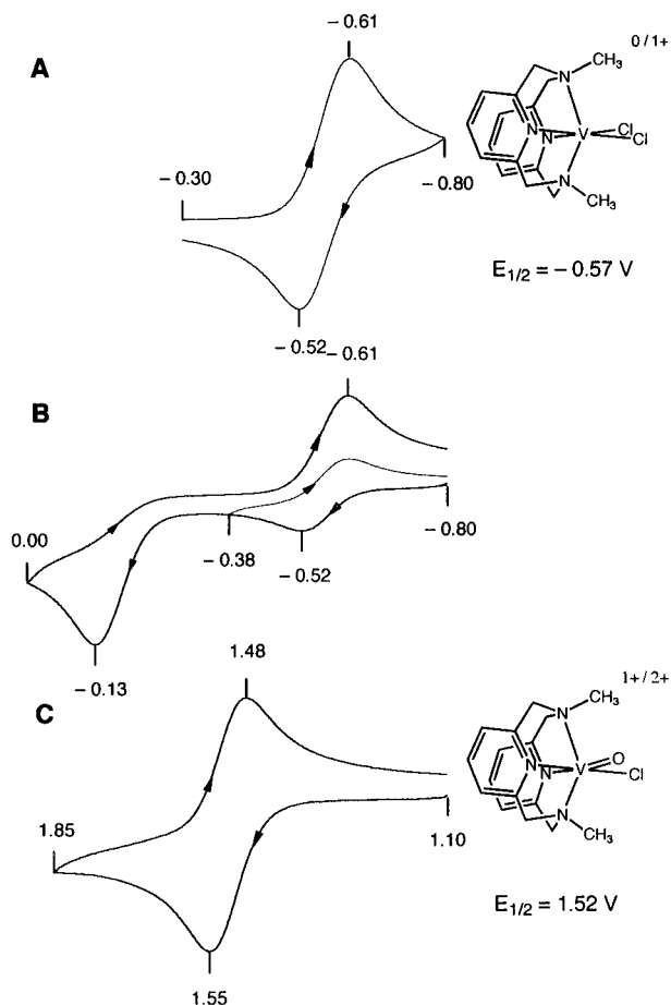
Figure 5. Cyclic voltammograms (A) of [(L-N 4 Me 2 )VCl 2 ](BPh 4 ) + (1) (200 mV/s), (B) of the product obtained by reducing [(L-N 4 Me 2 )VCl 2 ](BPh 4 ) + at -0.77\text{ V} (200 mV/s), and (C) of [(L-N 4 Me 2 )VClO](ClO 4 ) + (2) (50 mV/s) at a Pt-foil electrode in acetonitrile solutions at 25\text{ }^{\circ}\text{C} ; peak potentials and half-wave potentials vs SCE are indicated.
