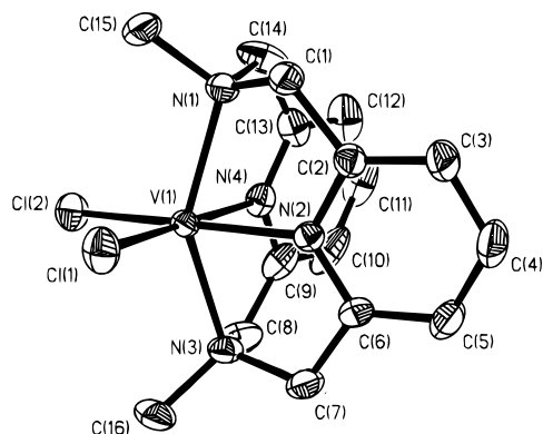
Figure 1. Structure of [(L-N 4 Me 2 )VCl 2 ] + showing thermal ellipsoids at 50% probability and the atom numbering scheme.
