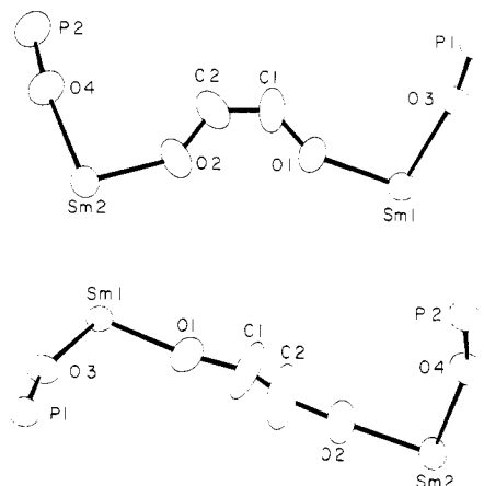
Figure 4. Comparison of the core atoms of cis - and trans - [(C_5Me_5)_2-[(C_6H_5)_3PO]Sm]_2(\mu-OCH=CHO) . The trans structure (bottom diagram) shows the large thermal ellipsoids for the bridge carbon atoms which would not refine to reasonable positions because of disorder.
