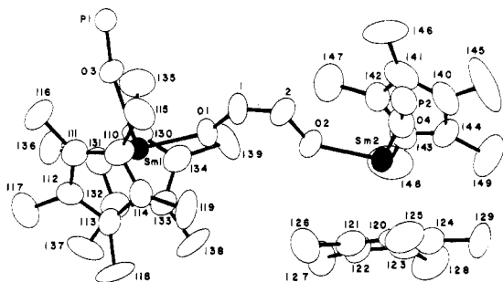
Figure 3. ORTEP drawing of cis - [(C_5Me_5)_2[(C_6H_5)_3PO]Sm]_2(\mu-OCH=CHO) (IIIa), with phenyl groups deleted. Carbon atoms are labeled with their numbers only.
