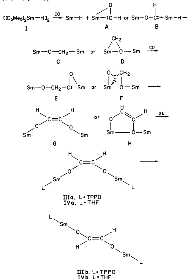
Scheme I. Possible Intermediates in the Formation of cis - and trans - \{(\text{C}_5\text{Me}_5)_2[(\text{C}_6\text{H}_5)_3\text{PO}]\text{Sm}\}_2(\mu\text{-OCH}=\text{CHO}) from \{(\text{C}_5\text{Me}_5)_2\text{SmH}\}_2 and CO a
