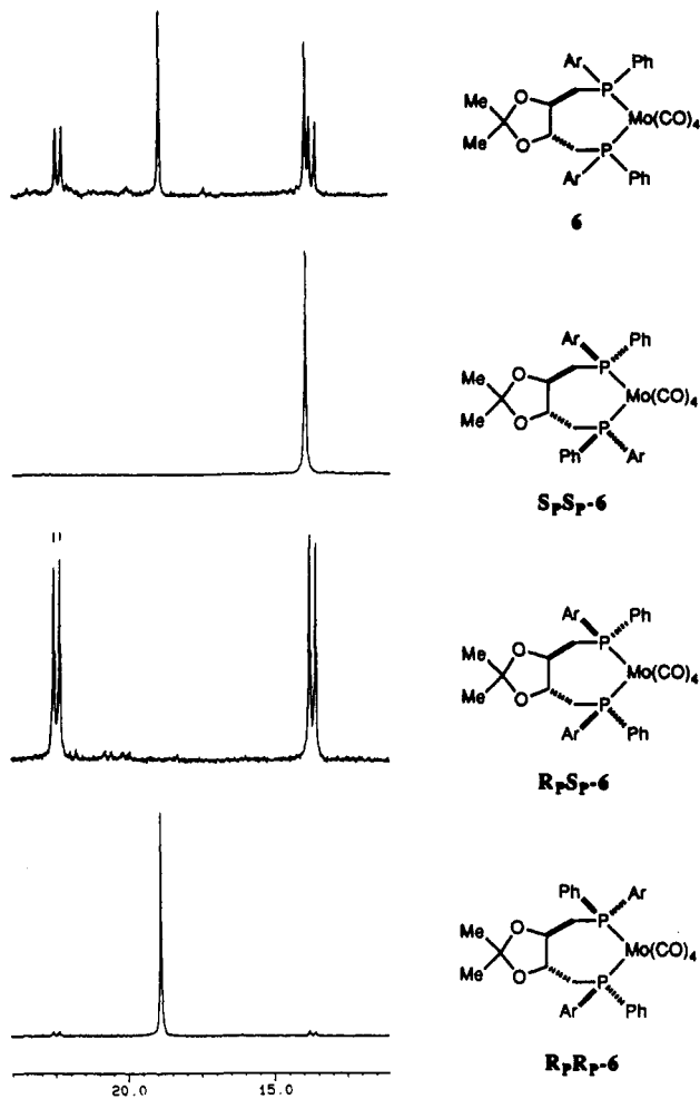
Figure 4. ^{31}\text{P} NMR data for diastereomeric complexes 6 ( \text{Ar} = 2\text{-MeOC}_6\text{H}_4 ).
