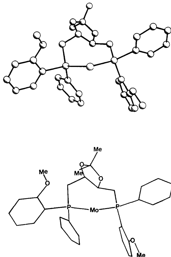
Figure 6. Crystal structure and schematic representation of ( R P , R P )-6 (carbonyl ligands omitted for clarity).
