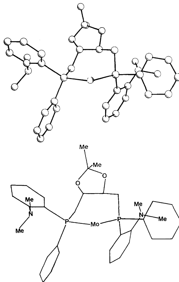
Figure 7. Crystal structure and schematic representation of ( R P , R P )-7 (carbonyl ligands omitted for clarity).
