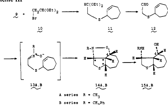
Scheme III
