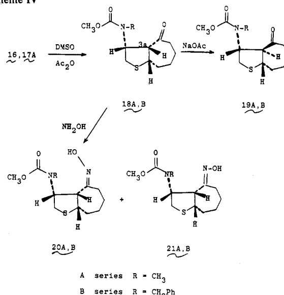
Scheme IV
