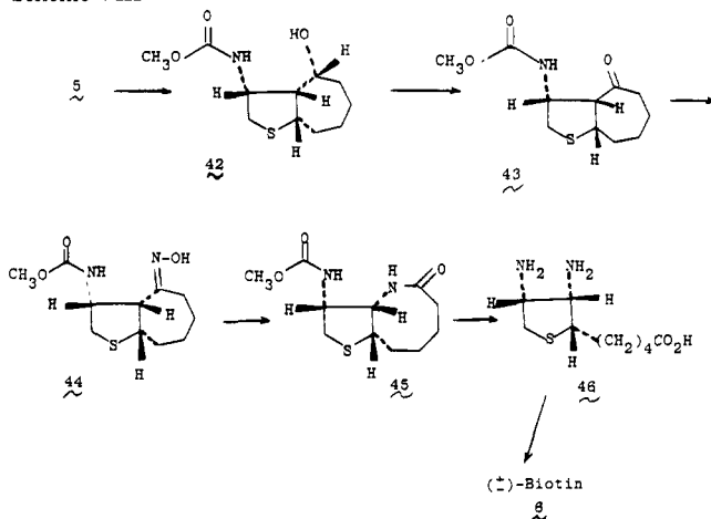
Scheme VIII
