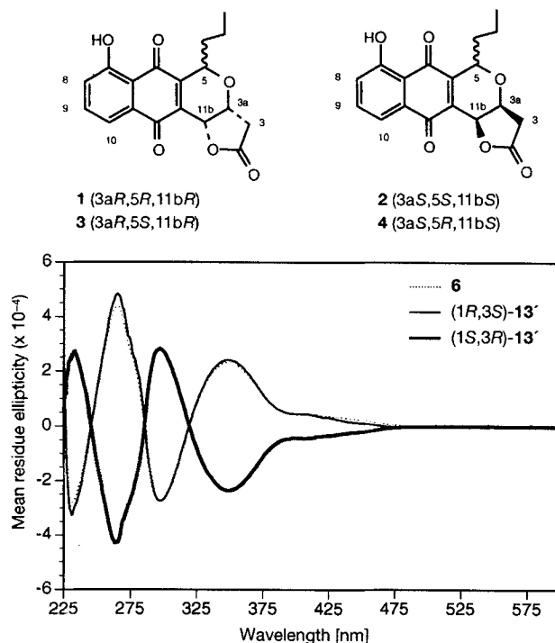
Fig. 3. ORD Spectra of (1 R ,3 S )- and of (1 S ,3 R )- 13' and of natural deoxyfrenolicin ( 6 )
