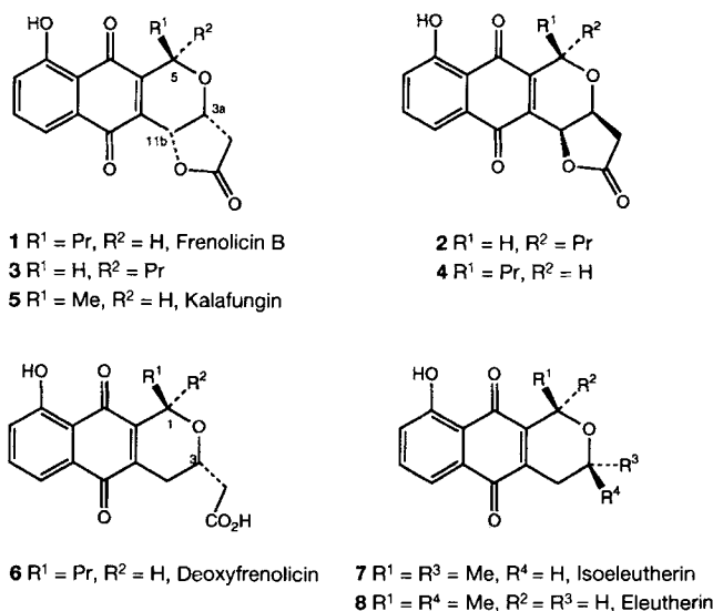
Fig. 1. Natural naphthopyranquinones containing an isochroman and a 1,4-naphthoquinone moiety
