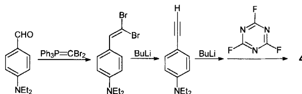
Scheme 2. Synthesis of 4.
