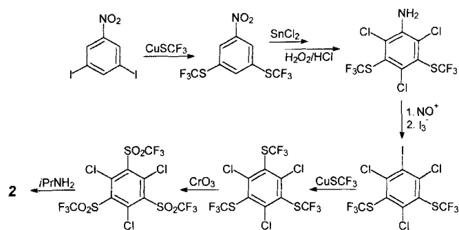
Scheme 1. Synthesis of 2 .
