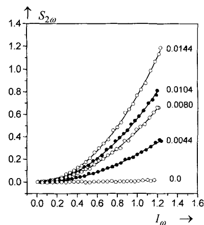
Figure 3. HRS signal S_{2\omega} (arb. units) as a function of the fundamental laser intensity I_\omega (arb. units) for dioxane solutions of 1 with mass fractions w = 0.0, 0.0044, 0.0080, 0.0104 , and 0.0144 . Each point represents an average over 300 laser pulses. The solid lines are quadratic fits.
