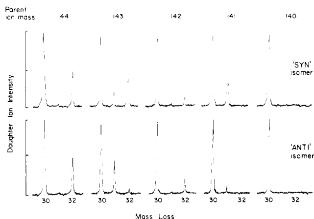
Figure 6. "Linked-scan" metastable ion mass spectra of the trimethylphosphate ions (the isotopically unlabeled ion has m/z of 140) that derive from the "syn" and "anti" cyclic triesters ( 10–12 ; 13–15 ) from the ( R )-phospho compound 36 (see Figure 5).
