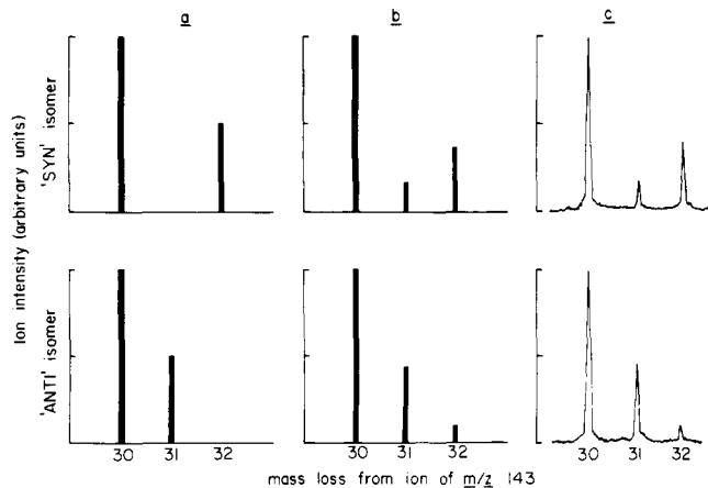
Figure 7. Metastable ion spectra for the (m + 3) ions at m/z 143 which come from the "syn" and "anti" cyclic triesters derived from 36 : (a) simplified spectra predicted for the fragmentation of the ion at m/z 143; (b) predicted spectra as in (a), taking into account the measured isomeric purity of the "syn" and "anti" cyclic triesters, the measured enantiomer excess of the starting diol, and the known contributions from the natural abundance of ^{13}\text{C} and ^2\text{H} ; (c) observed spectra.
