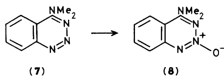
Scheme 1. Reagents: i, TFA/H 2 O 2 ; ii, H 2 /Pd/C
