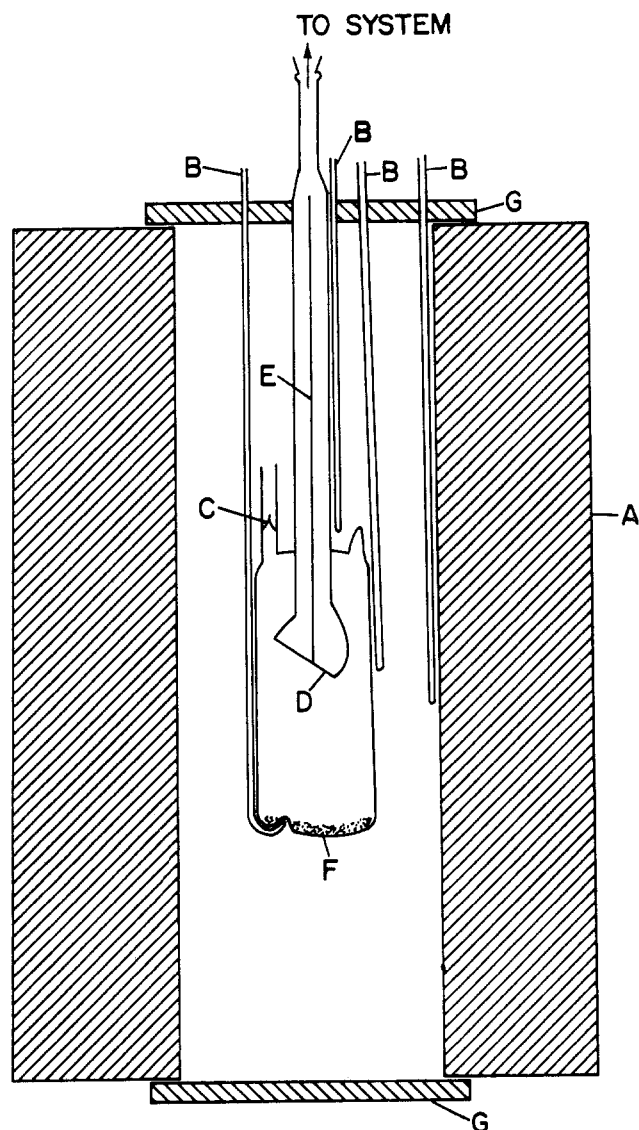
Fig. 2.—Diaphragm gage: A, Marshall furnace with external taps to furnace windings; B, thermocouples; C, fragile glass break-seal; D, glass diaphragm; E, null point indicator; F, solid \text{VBr}_3 .
