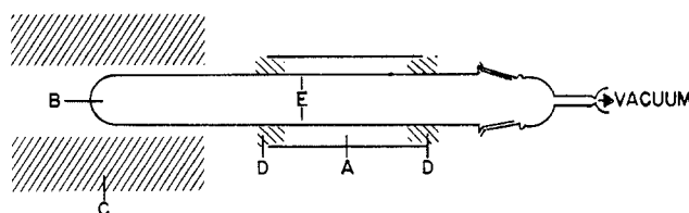
Fig. 3.—Apparatus for preparation of \text{VBr}_4 : A, solid \text{CO}_2 ; B, solid \text{VBr}_3 ; C, furnace; D, cork rings; E, condenser.
