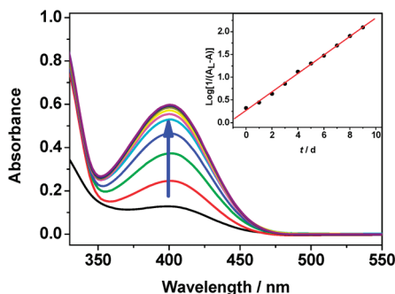
Figure 3. Family of UV–visible absorbance spectra of a 4-nitrophenoxy anion formed from the cleavage of BNPP in H 2 O at 50 °C. Inset: Kinetic plot of hydrolysis of BNPP using compound 1 as the catalyst. A is the observed absorbance, and A_L is the final absorbance at the end of the reaction.
