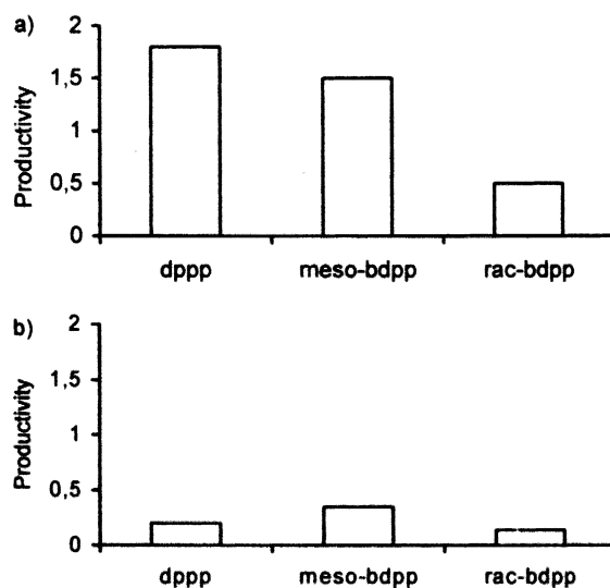
Figure 5. Productivity expressed as kg of polyketone ( \text{g of Pd}^{-1} ) vs chelating diphosphine ligand for the series of precursors (a) [\text{Pd}(\mu\text{-OH})(\text{P-P})_2](\text{PF}_6)_2 ; (b) [\text{Pd}(\text{P-P})_2](\text{PF}_6)_2 ( \text{P-P} = \text{dppp}, \text{meso-bdpp}, \text{rac-bdpp} ). Reaction conditions: solvent, \text{CH}_2\text{Cl}_2 ; time, 30 min.
