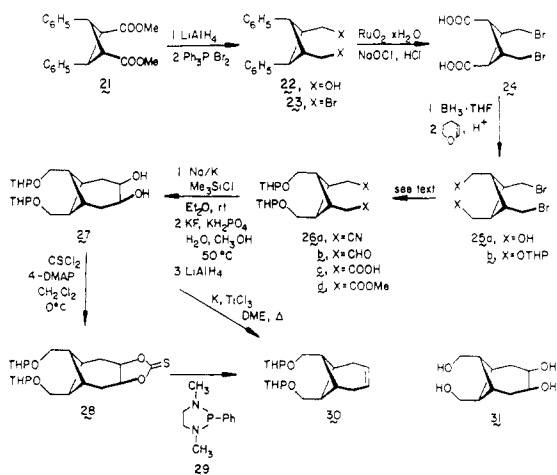
Scheme II
