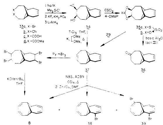
Scheme III
