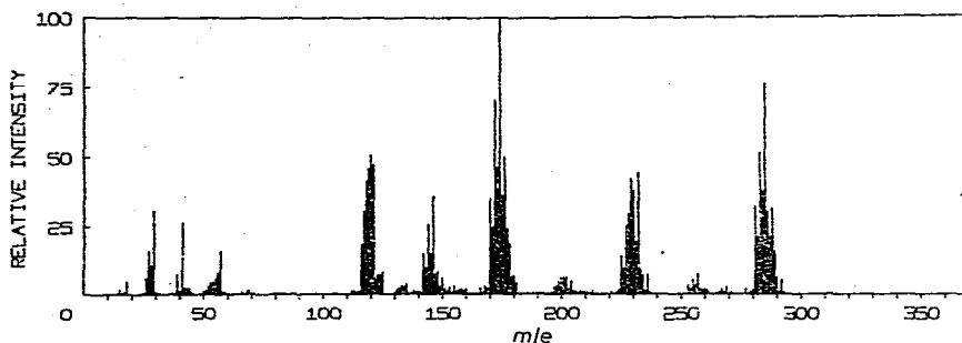
Fig. 4. (C_4H_9)_2Sn(CH_2CH_2CN)_2 .
