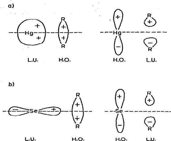
Fig. 7. Orbital interactions according to the perturbation model. The metal atoms are in their first excited states. a) Hg: ^1P b) Se: ^1D . R = alkyl, L.U. = lowest unoccupied, H.O. = highest occupied.
