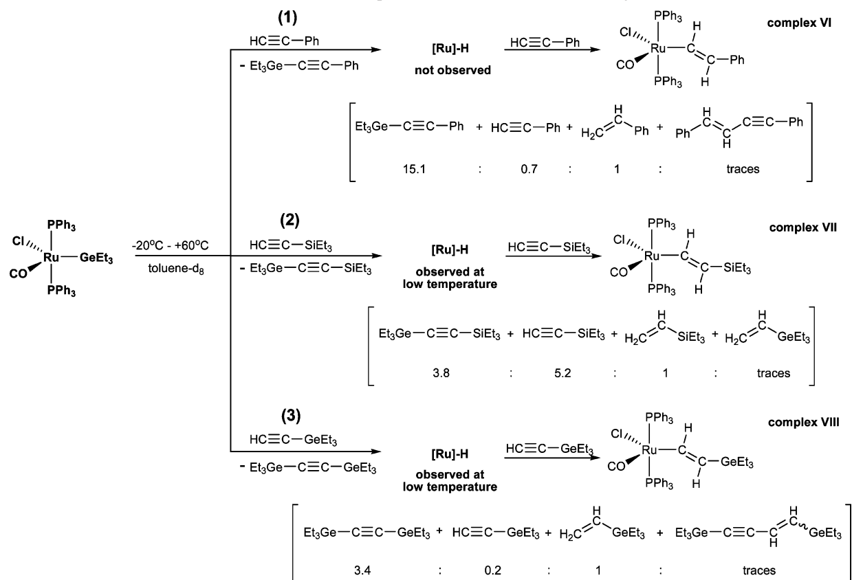
Scheme 3. Reaction of Equimolar Amounts of IV with Acetylenes
