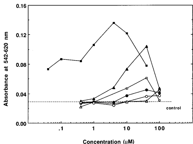
Figure 4. Effects of \beta -substituted 4-styrylpyridines and N^6 -benzyladenine on betacyanin biosynthesis by Amaranthus seedlings: Z -methylthio 8a (●), Z -ethoxy 8g (▲), Z -ethoxy N -oxide 8g (□), E -methylthio 9a (○), E -ethoxy (△), and N^6 -benzyladenine (■).
