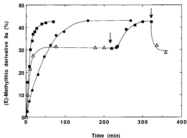
Figure 3. Cis-trans photoisomerization of Z -methylthio derivative 8a to its E -isomer 9a at different wavelengths. Compound 8a in \text{CDCl}_3 in a Pyrex NMR tube was irradiated at 280 (●), 320 (■), and 380 (△) nm, and Z/E ratios were determined by ^1\text{H} NMR at a given time. Arrows indicate the time at which the wavelength was changed.
