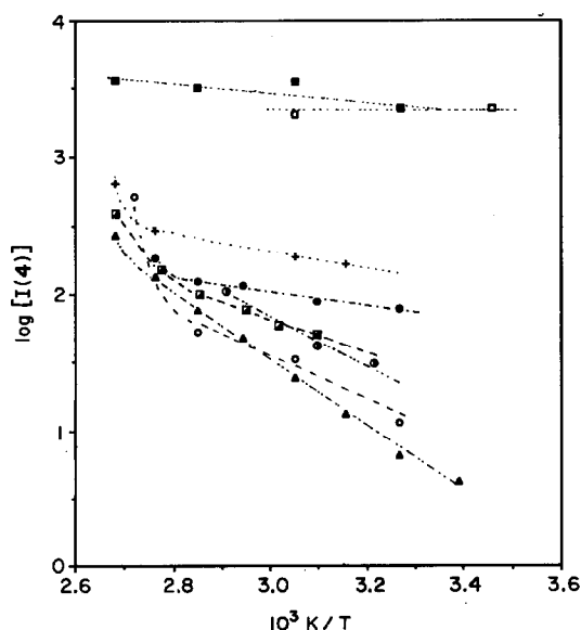
Fig. 1. Arrhenius type plot of spin adduct normalised signal intensities I (4). ▲ Et 2 Te, ● i Pr 2 Te, ● s Bu 2 Te, □ t Bu 2 Te, + (allyl) 2 Te, ▣ (benzyl) 2 Te, ○ i Pr 2 Te 2 , ■ t Bu 2 Te 2 .
