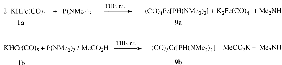
Scheme 4. Reaction of hydridocarbonylmetallates with \text{P}(\text{NMe}_2)_3 in the presence of a Brønstedt acid: \text{KHFe}(\text{CO})_4 itself in the case of iron, acetic acid in the case of chromium.
