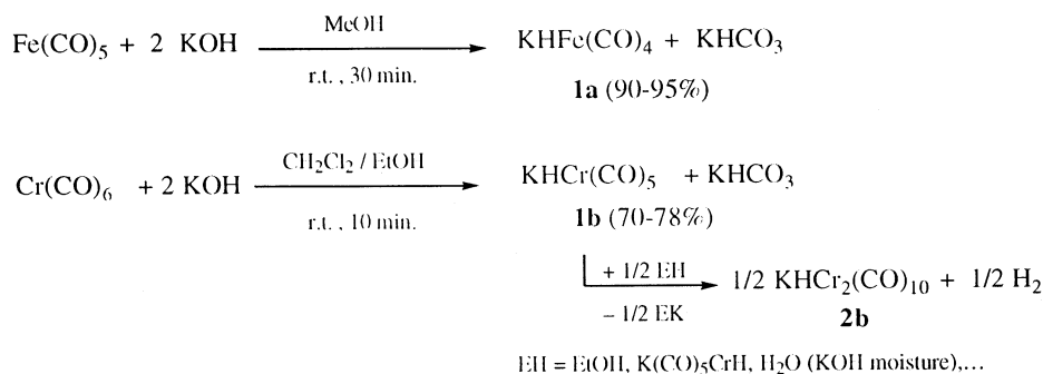
Scheme 1. Synthesis of mononuclear potassium hydridocarbonylmetallates.
