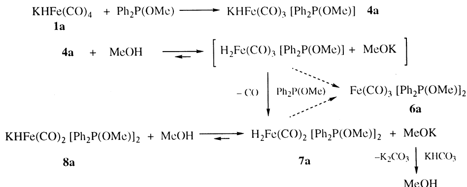
Scheme 3. Reaction of \text{Ph}_2\text{P}(\text{OMe}) with \text{KHFe}(\text{CO})_4 in methanol.
