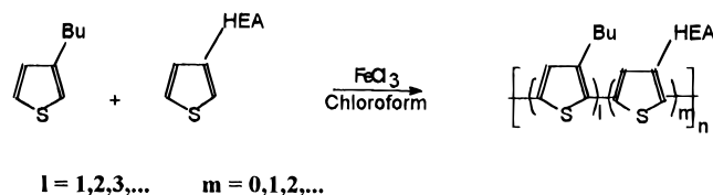
Figure 2. General polymerization of the copolymer 3-HEA-thiophene/3-butythiophene. The 3-HEA-thiophene monomers are randomly distributed.
