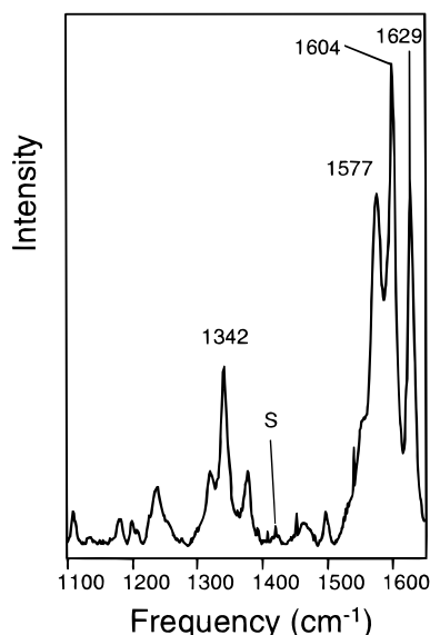
Figure 4. Resonance Raman spectrum of 4 ·Ni in \text{CH}_2\text{Cl}_2 (ca. 1 mM), measured with 457.9 nm CW excitation. S denotes solvent band.
