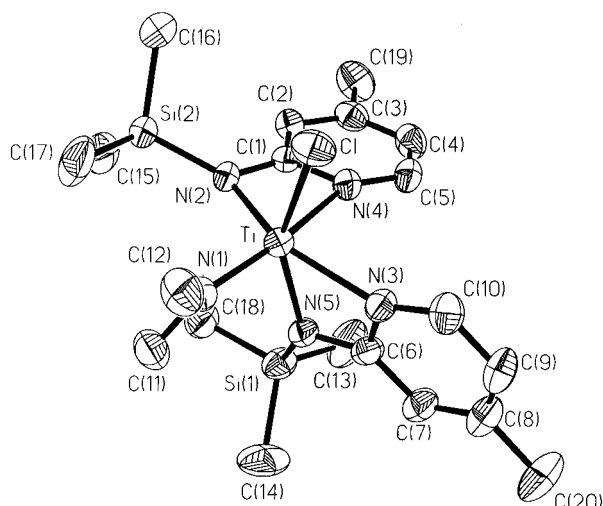
Figure 4. Structural representation of 2c . Hydrogen atoms are omitted for clarity. The thermal ellipsoids correspond to 40% probability. Selected bond distances (Å) and angles (deg): N(1)–Ti 1.892(3), N(2)–Si(2) 1.747(3), N(2)–Ti 2.031(3), N(3)–Ti 2.141(3), N(4)–Ti 2.220(3), N(5)–Si(1) 1.729(3), N(5)–Ti 2.096(3), Cl–Ti 2.3241(13), N(1)–Ti–N(2) 106.92(13), N(1)–Ti–N(5) 95.93(13), N(2)–Ti–N(5) 100.96(12), N(1)–Ti–N(3) 102.32(13), N(2)–Ti–N(3) 148.29(13), N(5)–Ti–N(3) 63.58(12), N(1)–Ti–N(4) 169.38(13), N(2)–Ti–N(4) 63.51(12), N(5)–Ti–N(4) 82.07(12), N(3)–Ti–N(4) 86.19(12), N(1)–Ti–Cl 96.10(10), N(2)–Ti–Cl 100.01(10), N(5)–Ti–Cl 151.58(10), N(3)–Ti–Cl 88.70(9), N(4)–Ti–Cl 90.37(9).
