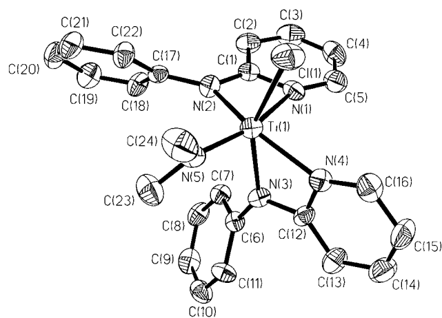
Figure 3. Structural representation of 2b . Hydrogen atoms are omitted for clarity. The thermal ellipsoids correspond to 40% probability. Selected bond distances (Å) and angles (deg): N(1)–Ti(1) 2.257(5), N(2)–Ti(1) 2.007(4), N(3)–Ti(1) 2.101(4), N(4)–Ti(1) 2.144(4), N(5)–Ti(1) 1.890(5), Cl(1)–Ti(1) 2.310(2), N(5)–Ti(1)–N(2) 99.9(2), N(5)–Ti(1)–N(3) 94.4(2), N(2)–Ti(1)–N(3) 99.4(2), N(5)–Ti(1)–N(4) 103.5(2), N(2)–Ti(1)–N(4) 151.2(2), N(3)–Ti(1)–N(4) 62.4(2), N(5)–Ti(1)–N(1) 161.6(2), N(2)–Ti(1)–N(1) 62.2(2), N(3)–Ti(1)–N(1) 85.2(2), N(4)–Ti(1)–N(1) 92.7(2), N(5)–Ti(1)–Cl(1) 99.5(2), N(2)–Ti(1)–Cl(1) 102.12(14), N(3)–Ti(1)–Cl(1) 151.85(13), N(4)–Ti(1)–Cl(1) 90.50(13), N(1)–Ti(1)–Cl(1) 89.02(12).
