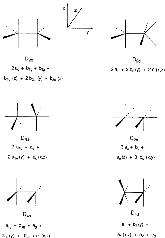
Fig. 6. Six possible structures for an unbridged \text{M}_2(\text{CO})_8 molecule. The point group and predicted normal \nu(\text{C}=\text{O}) vibrational modes are given for each structure, using the same set of cartesian axes in each case (as illustrated). The directions of the transition moment vectors for IR active modes are given in brackets.
