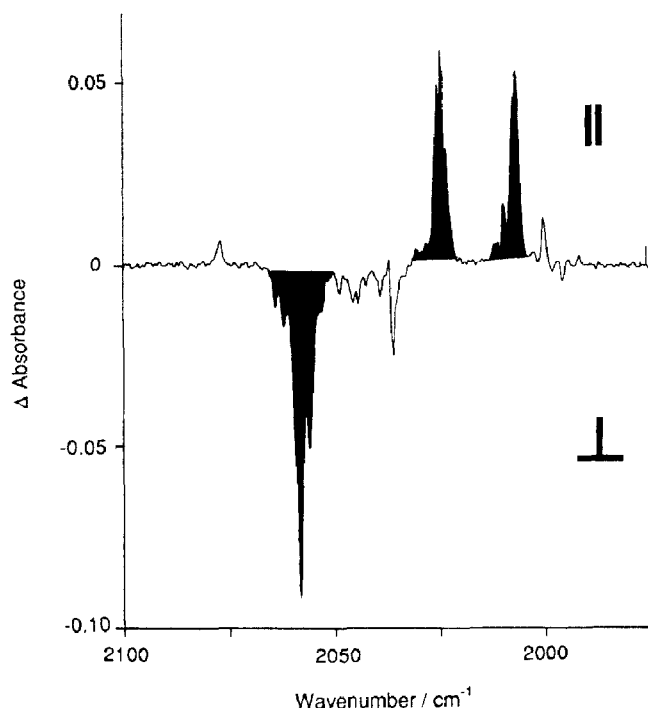
Fig. 7. IR difference spectrum ( \Delta absorbance = A_{||} - A_{\perp} ) showing the dichroism generated by 10 min irradiation of a randomly oriented sample of \text{Os}_2(\text{CO})_8 in a \text{N}_2 matrix with plane polarised light ( > 525 nm). The polarisations of the bands of the remaining \text{Os}_2(\text{CO})_8 are the opposite to those observed in Fig. 4b (see text for discussion).
