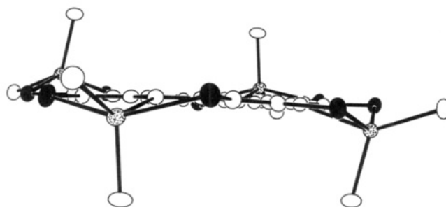
Figure 3. ORTEP diagram of 7a , emphasizing the planarity of the porphyrazineoctathiolato ligand. Sulfur atoms are drawn in black and tin atoms are shaded. Methyl groups are omitted for clarity.
