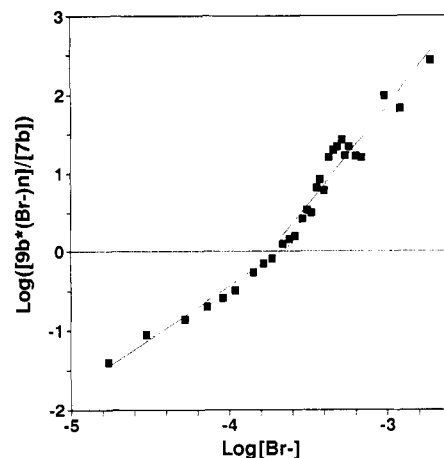
Figure 8. Plot of the logarithm of the reaction coordinate \{\log ([\mathbf{9b} \cdot \text{Br}_n]/[\mathbf{7b}]_{\text{total}})\} versus \log [\text{Br}^-] as monitored by the increase in absorbance maximum at 338 nm.
