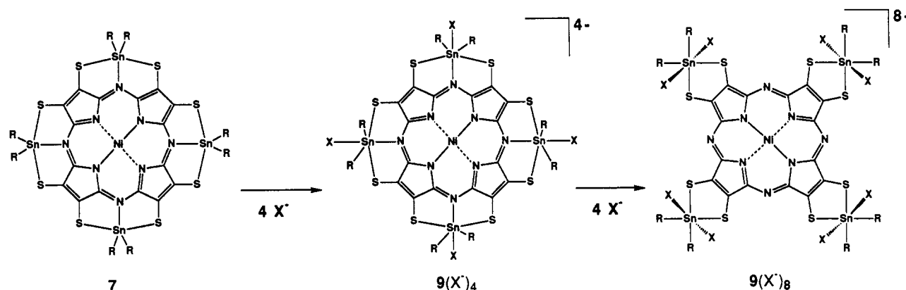
Scheme II
