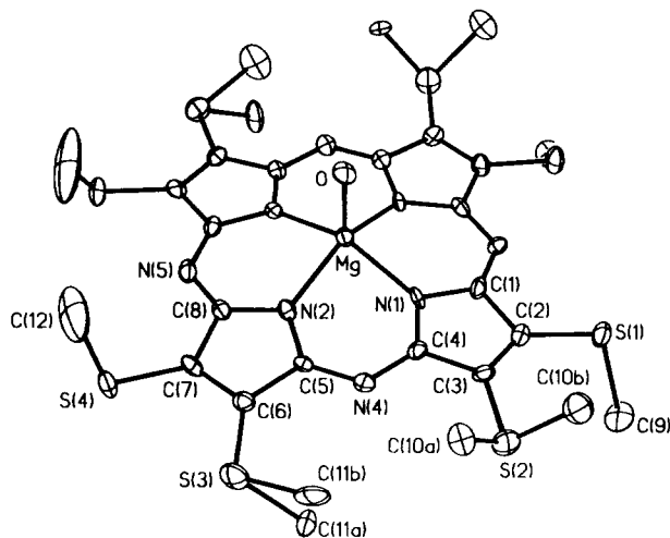
Figure 4. ORTEP diagram of 3b ·H 2 O with hydrogen atoms omitted for clarity. The disorder in C10 and C11 is modeled using two sites (a and b) for each atom.
