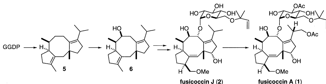
Scheme 2. The metabolic process from geranylgeranyl diphosphate (GGDP) to fusicoccins in Phomopsis ( Fusicoccum ) amygdali
