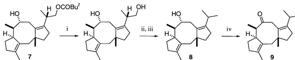
Scheme 3. Reagents and conditions. (i) \text{LiAlH}_4 , THF (100%); (ii) \text{TsCl} , Py; (iii) \text{LiEt}_3\text{BH} , THF (two steps, 20%); † (iv) P. amygdali , 3 days (ca. 30%)
