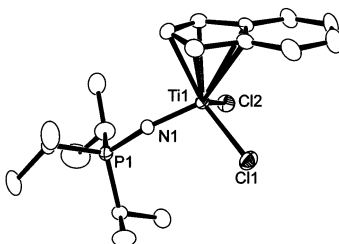
Figure 3. ORTEP drawing of 23 , 30% thermal ellipsoids, H atoms omitted for clarity.
