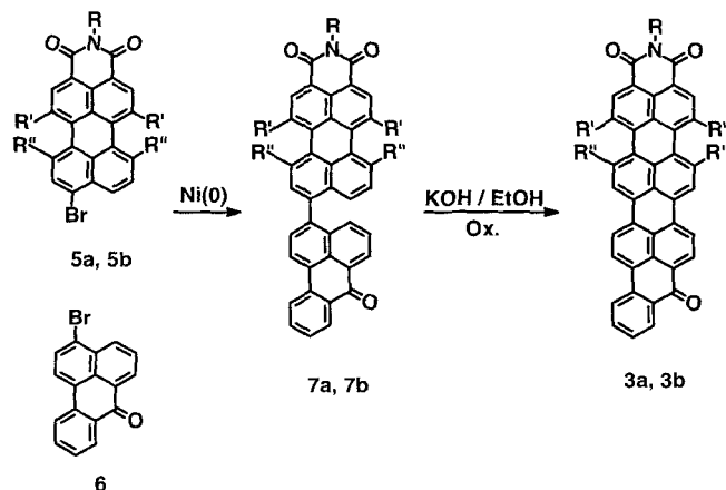
Scheme 2. Syntheses of benzoylterrylenedicarboximide 3a and 3b (a: \text{R} = n\text{-propyl} , \text{R}' = \text{R}'' = 4\text{-tert-butylphenoxy} ; b: \text{R} = 2,6\text{-diisopropylphenyl} , \text{R}' = 4\text{-tert-butylphenoxy} , \text{R}'' = \text{H} ). Reagents, conditions, and yields: a) 7a : \text{Ni}(\text{PPh}_3)_2\text{Cl}_2 , \text{Zn} , \text{NEt}_4/\text{THF} , 25^\circ\text{C} , 12 h/45%; 7b : \text{Ni}(\text{cod})_2 , cod, bipy/DMF, 70^\circ\text{C} , 2 d/62%; b) \text{KOH} , ox./EtOH, 70^\circ\text{C} , 15 min/80%.
