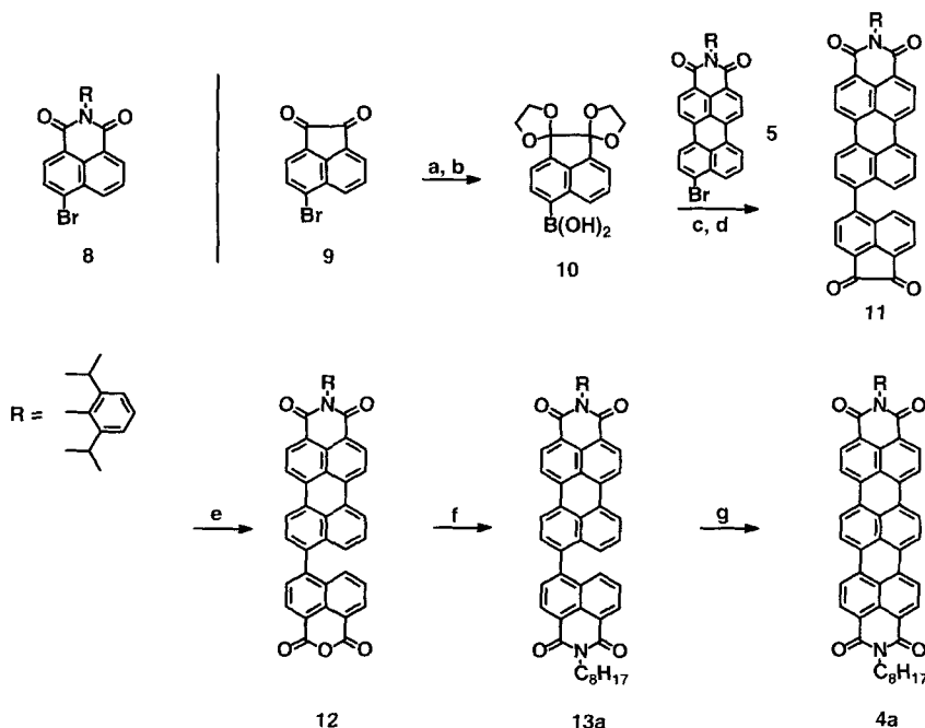
Scheme 3. Synthesis of terrylenetetracarboxydiimide 4a : reagents, conditions, yields: a) ethyleneglycol, conc. \text{H}_2\text{SO}_4/m\text{-xylene} , reflux, 4 d/85%; b) 1. n\text{-butyllithium}/\text{THF} , -78^\circ\text{C} ; 2. triisopropylborate/THF, -78^\circ\text{C} ; 3. \text{H}_2\text{O}/60\% . c) [\text{Pd}(\text{PPh}_3)_4] , 2M \text{K}_2\text{CO}_3/\text{toluene} , reflux, 20 h/75%; d) \text{H}_2\text{SO}_4 , \text{H}_2\text{O}/1\text{-PrOH} , reflux, 4 d/>95%; e) \text{KOH} , \text{O}_2/1\text{-PrOH} , 60^\circ\text{C} , 4 h/>95%; f) n\text{-octylamine}/2\text{-PrOH} , reflux, 10 h/>95%; g) \text{KOH} , ox./EtOH, 70^\circ\text{C} , 15 min/80%.
