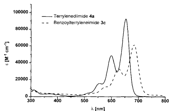
Figure 1. Absorption spectra of 3c and 4a ( \text{CHCl}_3 ).
