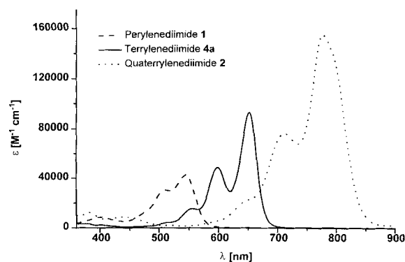
Figure 2. Absorption spectra of 1 , 4a , and 2 ( \text{CHCl}_3 ).
