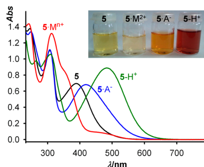
Figure 4. Changes in the absorption spectra of 5 (black) ( c = 5 \times 10^{-5} M in CH 3 CN) upon addition of increasing amounts of: Pb(ClO 4 ) 2 ; Zn(OTf) 2 and Hg(OTf) 2 (deep red); [(n-Bu) 4 N]AcO, [(n-Bu) 4 N] 2 SO 4 and [(n-Bu) 4 N]H 2 PO 4 (deep blue); [(n-Bu) 4 N]F, [(n-Bu) 4 N] 3 HP 2 O 7 and [(n-Bu) 4 N]OH (deep green). Inset: visual features observed upon addition of metal cations, anions, and upon deprotonation.
