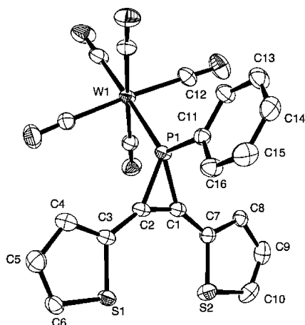
Figure 1. Molecular structure of the 2,3-dithienylphosphirene pentacarbonyltungsten complex ( 1 ). Main bond lengths (Å) and angles (deg): P–W 2.4853(6), P–C(11) 1.828(2), P–C(1) 1.788(2), P–C(2) 1.787(2), C(1)–C(2) 1.324(3), C(2)–C(3) 1.431(3), C(3)–S(1) 1.729(2), C(6)–S(1) 1.707(2); C–P–C 43.5(1).
