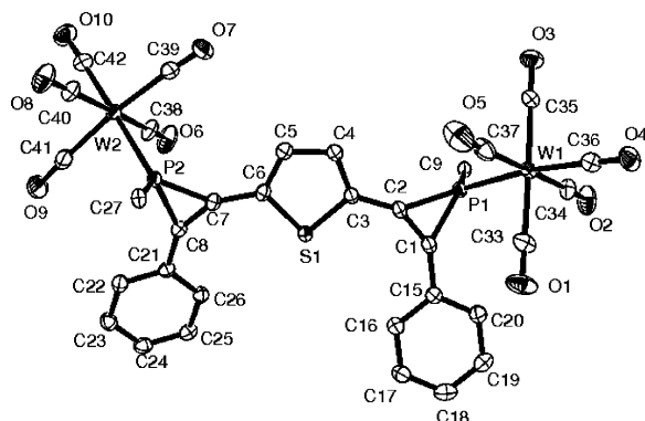
Figure 4. Molecular structure of the ( S,S )-enantiomer of rac -6. Phenyl substituents at P are omitted for clarity. Main bond lengths (Å) and angles (deg): W(1)–P(1) 2.489(1), P(1)–C(1) 1.787(4), P(1)–C(2) 1.804(4), P(1)–C(9) 1.810(4), C(1)–C(2) 1.332(5), C(1)–C(15) 1.453(5), C(3)–S(1) 1.725(4), C(2)–C(3) 1.429(5), C(3)–C(4) 1.372(5), C(4)–C(5) 1.409(5); C(2)–P(1)–C(1) 43.5(2), C(2)–C(1)–P(1) 68.9(2), C(1)–C(2)–P(1) 67.5(2), P(1)–C(2)–C(3) 145.6(3), P(1)–C(1)–C(15) 145.0(3), C(1)–P(1)–C(9) 108.5(2), C(1)–P(1)–W(1) 124.1(1), C(3)–S(1)–C(6) 91.7(2), S(1)–C(3)–C(2) 120.7(3), S(1)–C(3)–C(4) 111.3(3).
