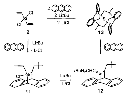
Scheme 4. Reactions of dichlorodivinylsilane with Li t Bu and anthracene.
