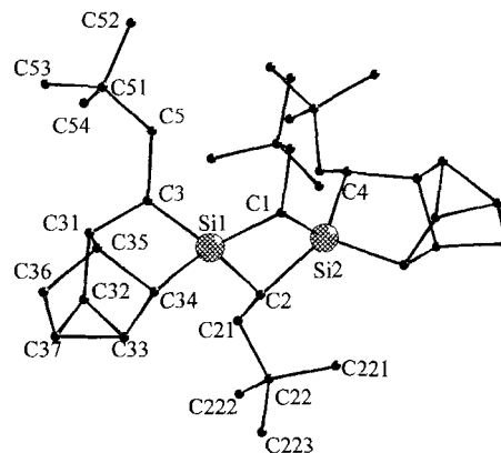
Figure 4. DIAMOND plot of the molecular structure of 17 .
