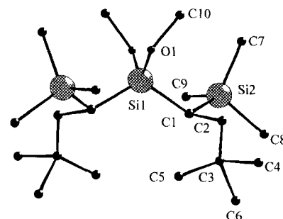
Figure 1. DIAMOND plot of the molecular structure of 10 .
