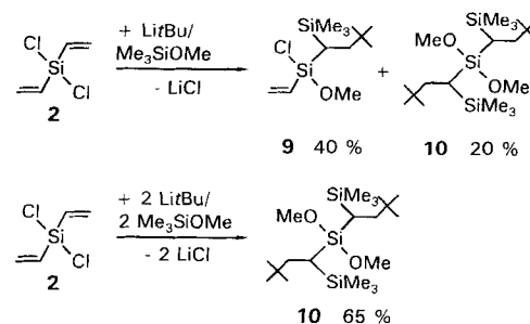
Scheme 3. Trapping reactions of dichlorodivinylsilane with Li t Bu and Me 3 SiOMe.
