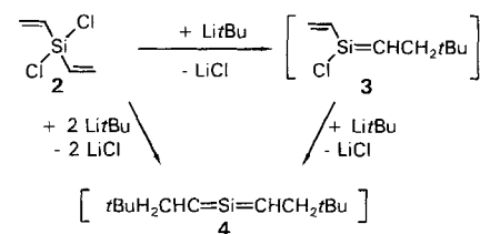
Scheme 1. Reactions of dichlorodivinylsilane with one or two equivalents of \text{Li}t\text{Bu} .
