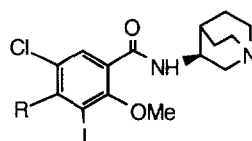
3 , R = H 4 , R = NH 2
