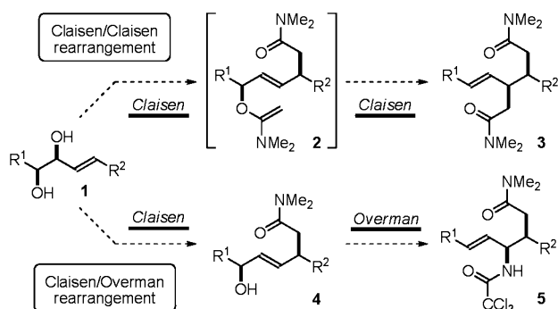
Scheme 1. Two Types of Sequential Sigmatropic Rearrangements
