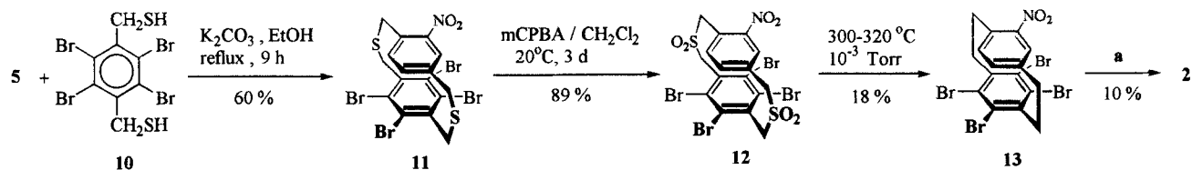
Scheme 2. Synthesis of 2
