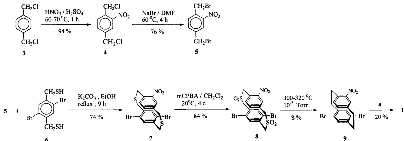
Scheme 1. Synthesis of 1
