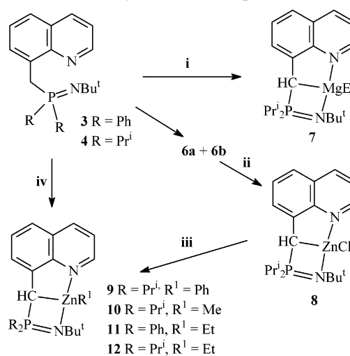
Scheme 2. Synthesis of Complexes 7–12 a
