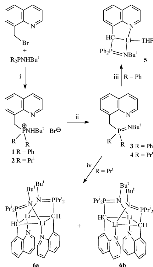
Scheme 1. Synthesis of Compounds 1–6 a
