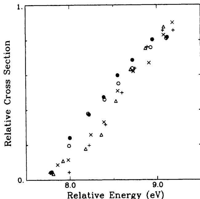
Figure 1. The relative cross section for butyl iodide reacting with tetraakis(dimethylamino)ethylene is plotted against the relative translational energy: (O) tert -butyl iodide, ( \Delta ) sec -butyl iodide, (+) n -butyl iodide, ( \times ) isobutyl iodide. The open and closed circles are two separate runs. The cross sections were scaled by the following factors: tert -butyl iodide, 1.00; sec -butyl iodide, 0.44; n -butyl iodide, 0.31; and isobutyl iodide, 0.31. The relative cross section is given by the ordinate of the figure times the scaling factor. The butyl iodide beam was held at 26 °C, while the temperature of the TDMAE beam was varied over a range of 40–300 °C to obtain the range of translational energies.
