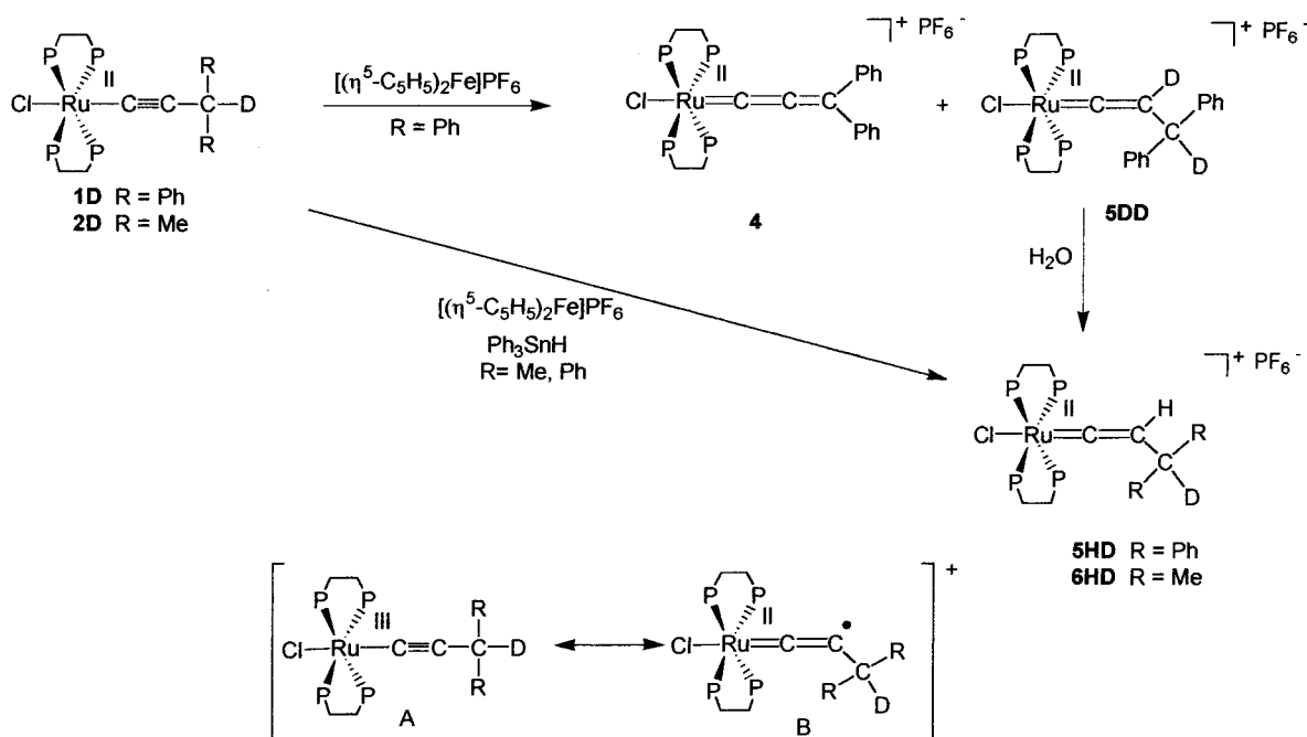
Scheme 3
