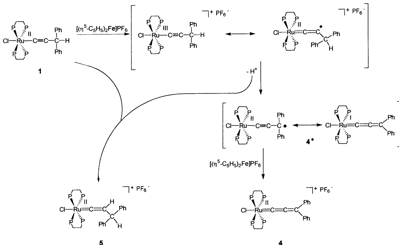
Scheme 4
