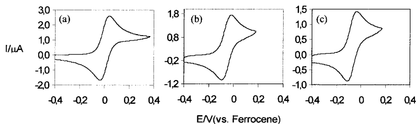
Figure 1. Cyclic voltammetry responses ( \text{CH}_2\text{Cl}_2 , \text{Bu}_4\text{NPF}_6 0.1 M, \nu = 100 \text{ mV s}^{-1} ) reported vs internal ferrocene for (a) trans - [\text{Cl}(\text{dppe})_2\text{Ru}-\text{C}\equiv\text{C}-\text{CHPh}_2] ( 1 ), (b) trans - [\text{Cl}(\text{dppe})_2\text{Ru}-\text{C}\equiv\text{C}-\text{CH}(\text{CH}_3)_2] ( 2 ), and (c) trans - [\text{Cl}(\text{dppe})_2\text{Ru}-\text{C}\equiv\text{C}-\text{CH}_3] ( 3 ).
