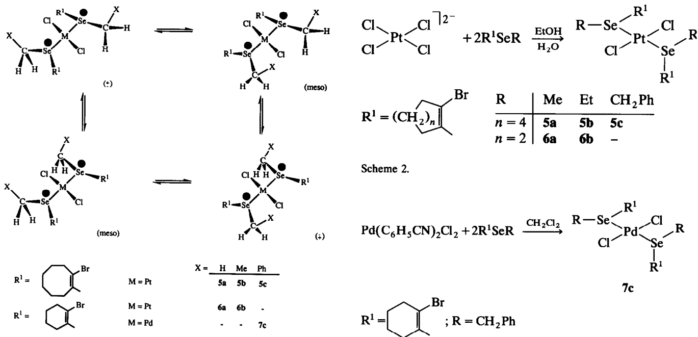
Fig. 1. Interconversion of isomers of 5a–c , 6a, b and 7c via inversion of selenium.
