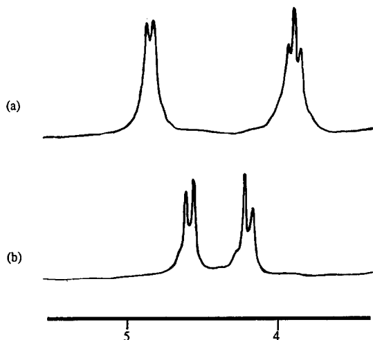
Fig. 2. ^1\text{H} NMR spectra (methylene region) of (a) 5c ; (b) 7c .
