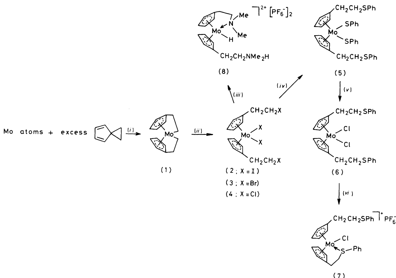
Scheme. (i) -196^{\circ}\text{C} (50–60%); (ii) X = Cl: Cl 2 in light petroleum (b.p. 60-80^{\circ}\text{C} ) for 15 min (30%) or PhICl 2 in thf (90%); X = Br: Br 2 in light petroleum (b.p. 60-80^{\circ}\text{C} ) (60%); X = I: I 2 in thf (95%); (iii) NHMe 2 in thf at 56^{\circ}\text{C} then NH 4 PF 6 , (76%); (iv) NaSPh in ethanol, reflux for 5 h (87%); (v) HCl gas in CH 2 Cl 2 for 1 h (83%); (vi) FeCl 2 in thf at 50^{\circ}\text{C} for 1 h (37%)
