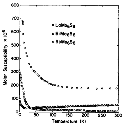
FIG. 1. The molar susceptibility of MeMo_6X_8 ( Me = La, Bi, \text{ and } Sb ) as a function of temperature.
