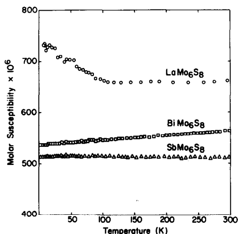
FIG. 2. The molar susceptibility of MeMo_6X_8 ( Me = La, Bi, \text{ and } Sb ) corrected for diamagnetic cores and paramagnetic impurities as a function of temperature.
