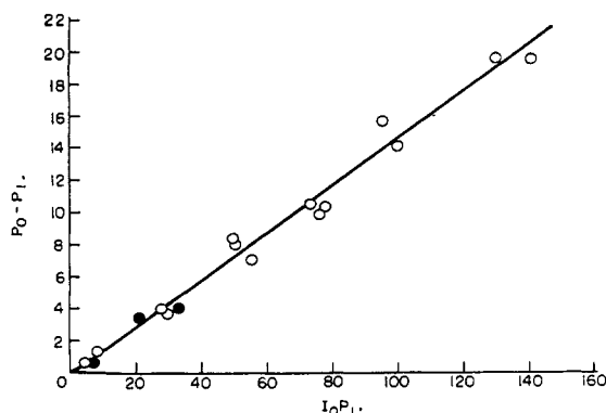
Fig. 1.—Acetone decomposed.
