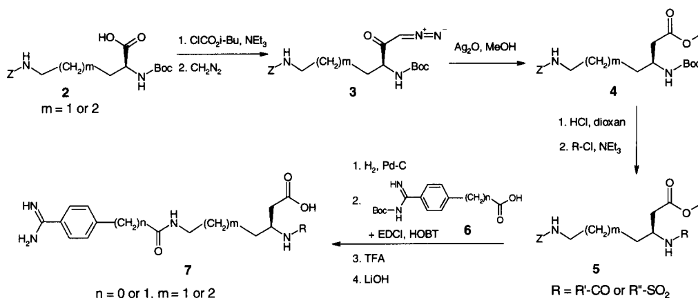
Scheme 1. Preparation of beta-amino acid GPIIb/IIIa antagonists
