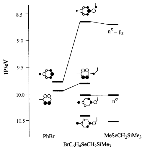
Fig. 7. Correlation of molecular orbitals upon the formation of \text{BrC}_6\text{H}_4\text{SeCH}_2\text{SiMe}_3 .
