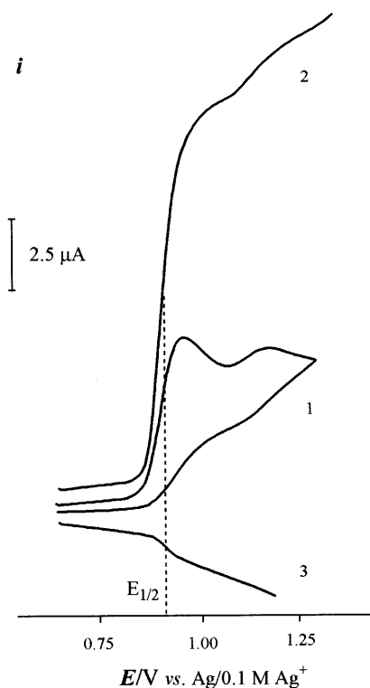
Fig. 1. Oxidation of arylselenide 1c ( C = 10^{-3} \text{ mol l}^{-1} , T = 20^\circ\text{C} ) in \text{CH}_3\text{CN}-0.01 \text{ M Et}_4\text{NClO}_4 . (1) Cyclic voltammogram, v = 0.5 \text{ V s}^{-1} ; (2) and (3) are curves registered at a Pt rotating disk electrode, \omega = 20 \text{ s}^{-1} , (2) classical curve, (3) commutated curve with the connection according to the second scheme; switch frequency f = 100 \text{ Hz} , capacitive current reduced.
