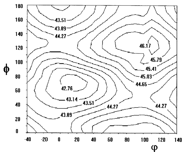
Fig. 5. Diagram of MMX energy of the molecule 1b as a function of two torsion angles: ( \varphi ) \angle \text{C}_{\text{sp}2}(2)\text{--C}_{\text{sp}2}(1)\text{--Se--C}_{\text{sp}3} and ( \phi ) \angle \text{C}_{\text{sp}2}(1)\text{--Se--C}_{\text{sp}3}\text{--Si} .
