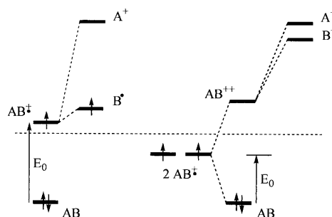
Fig. 2. Correlation of frontier orbitals in first and second order potential-determining reactions of cation radicals \text{AB}^{\bullet+} . Left: charge-controlled cleavage of the cation radical; right: fragmentation of a dication \text{AB}_2^{\bullet+} preceded by an orbital-controlled disproportionation of cation radicals. The orbital energy corresponds to the direction of ordinate axes so the presentation of orbitals is turned upside down. Horizontal dotted line designates the energy level which delimits charge- and orbital-controlled interactions of cation radicals.
