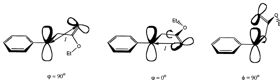
Fig. 11. Rotation about C_{sp3}-C(O) and the Se-C_{sp3} bonds favoring shortest Se\cdots O interatomic distance l (torsion angle \varphi ) and frontal orientation of interacting orbitals (torsion angle \phi ).
