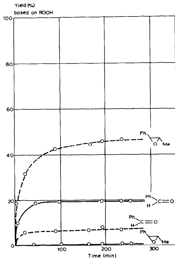
Fig. 5. Oxidation of trans - \beta -methyl styrene by t -BuOOH or \text{Ph}_3\text{COOH} catalyzed by 1a . [ 1a ] 0.02 M ; solvent, \text{CH}_2\text{Cl}_2 ; temperature, 20°C; olefin/complex = 70; ROOH/complex = 20. — — — t -BuOOH, — \text{Ph}_3\text{COOH} .
