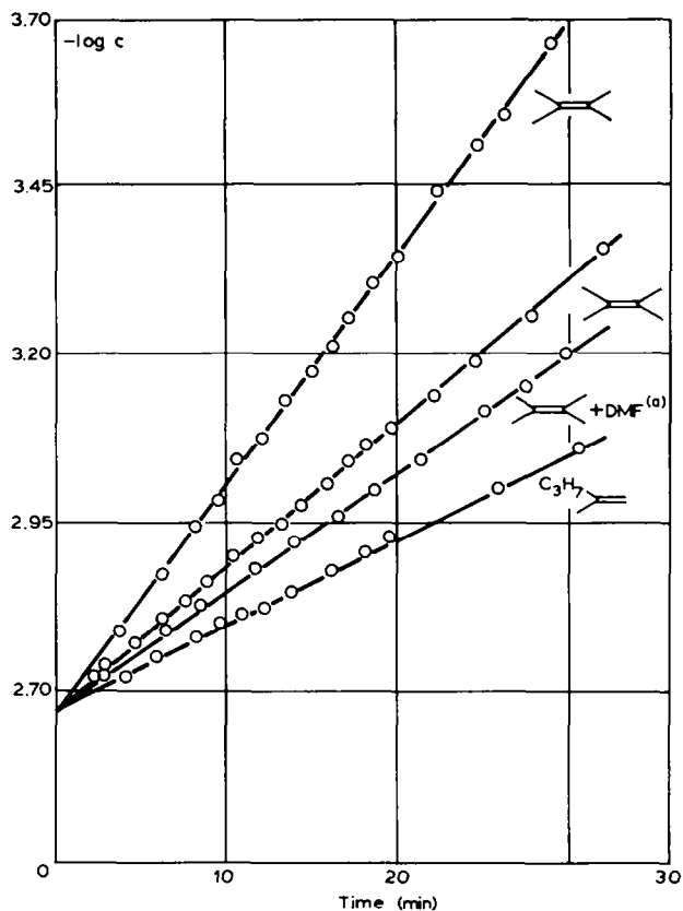
Fig. 3. Oxidation of olefins by IIIa. First order plot of \log [\text{IIIa}] vs. time. temperature, 20°C: [\text{IIIa}] 2.1 \times 10^{-3} M ; olefin/complex = 40; solvent, \text{CH}_2\text{Cl}_2 . a \text{DMF} = 3.5 \times 10^{-3} M .
