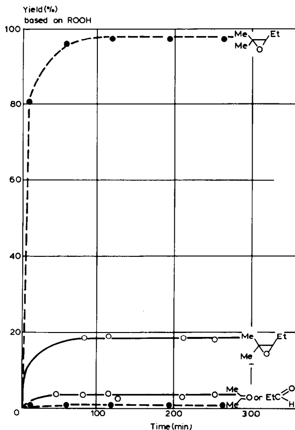
Fig. 4. Oxidation of 2-methyl-2-pentene by t -BuOOH or Ph 3 COOH catalysed by Ia. ● t -BuOOH, ○ Ph 3 COOH; [Ia] 0.02 M ; solvent, CH 2 Cl 2 ; temperature, 20°C; ROOH/complex = 20; olefin/complex = 70.
