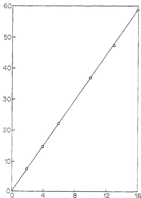
Figure 2. Aminolysis rates of p -nitrophenyl decanoate by n -decylamine at zero buffer concentration (by extrapolation of Figure 1): ordinate, 10%(aminolysis rate) ( M \text{ min}^{-1} ); abscissa, 10%(free amine concentration) ( M ).
